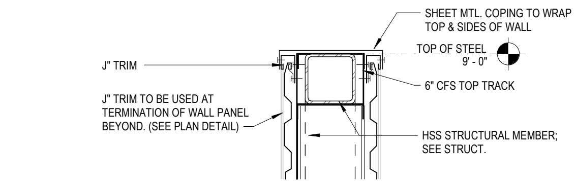
3 DETAIL @ TOP OF PRIVACY WALL 1 1/2" = 1'-0"
