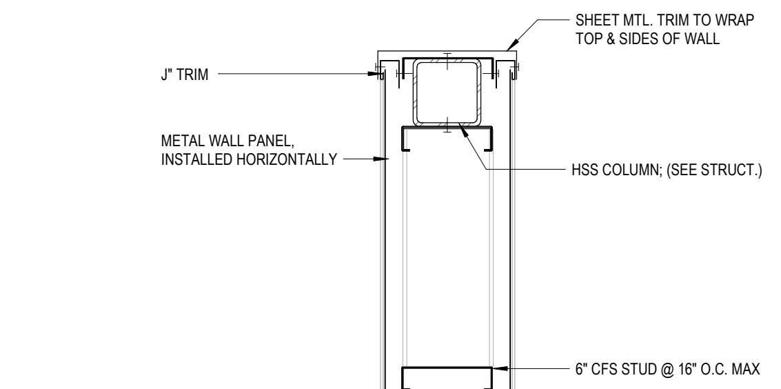
4 PLAN DETAIL @ PRIVACY WALL 1 1/2" = 1'-0"
