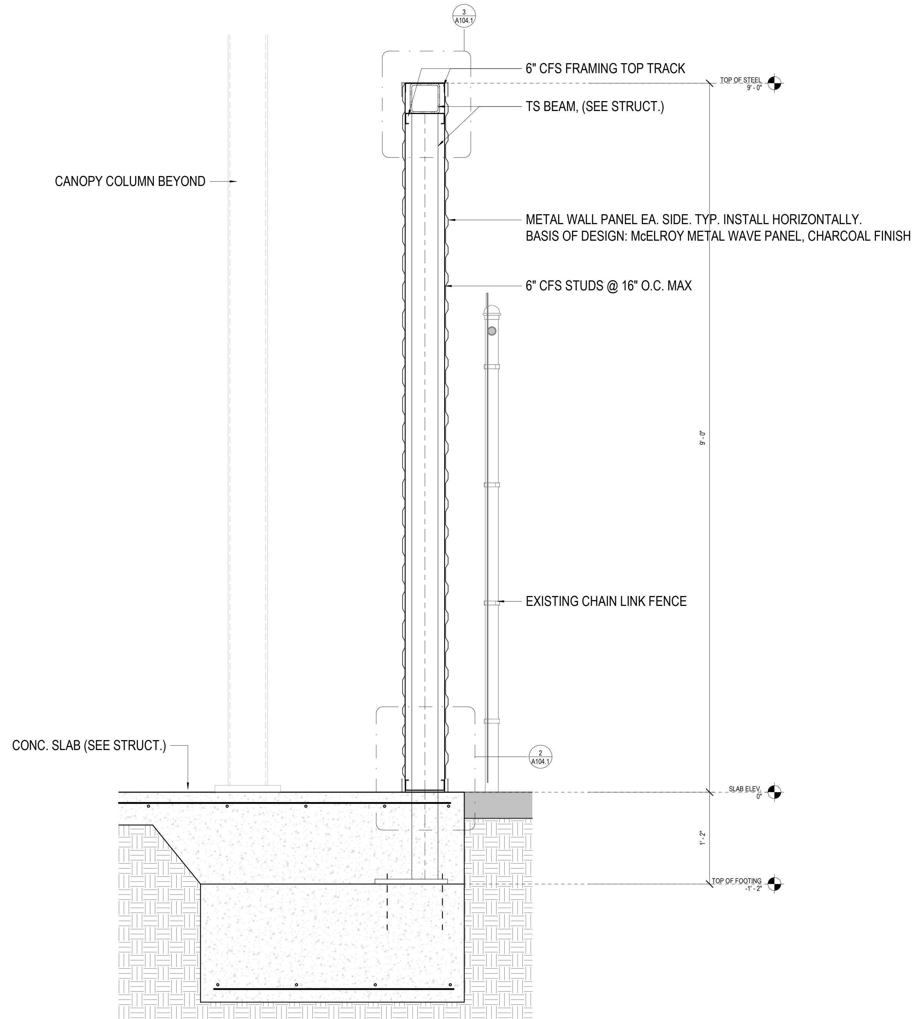
1 SECTION DETAIL @ PRIVACY WALL 1 1/2" = 1'-0"
