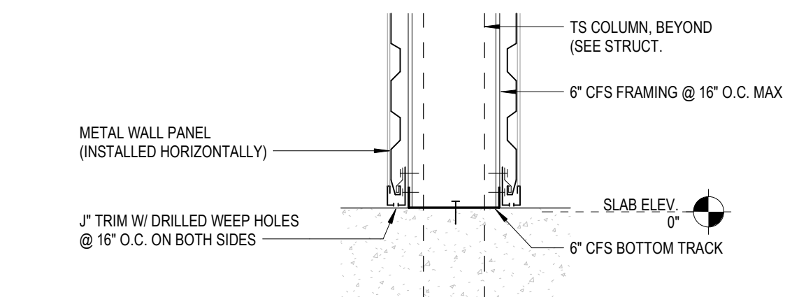
2 DETAIL @ BASE OF PRIVACY WALL 1 1/2" = 1'-0"
