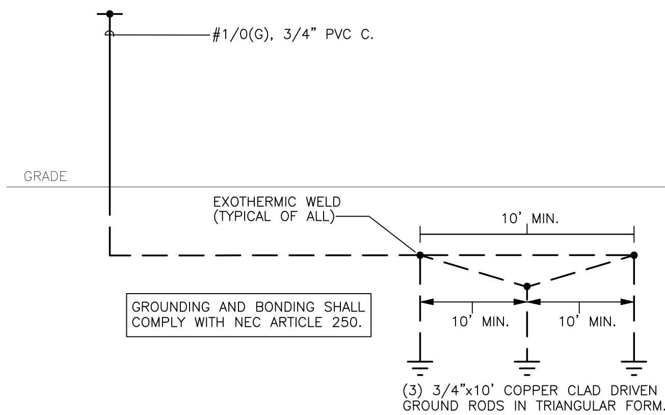
2 GROUNDING DETAIL Scale: NONE
