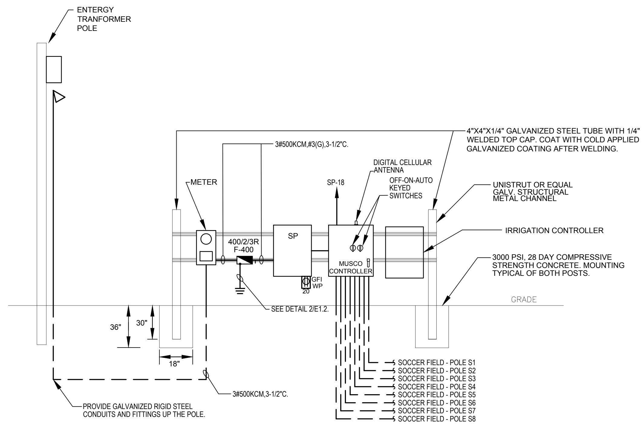
3 SINGLE LINE DIAGRAM - SOCCER FIELDS Scale: NONE
