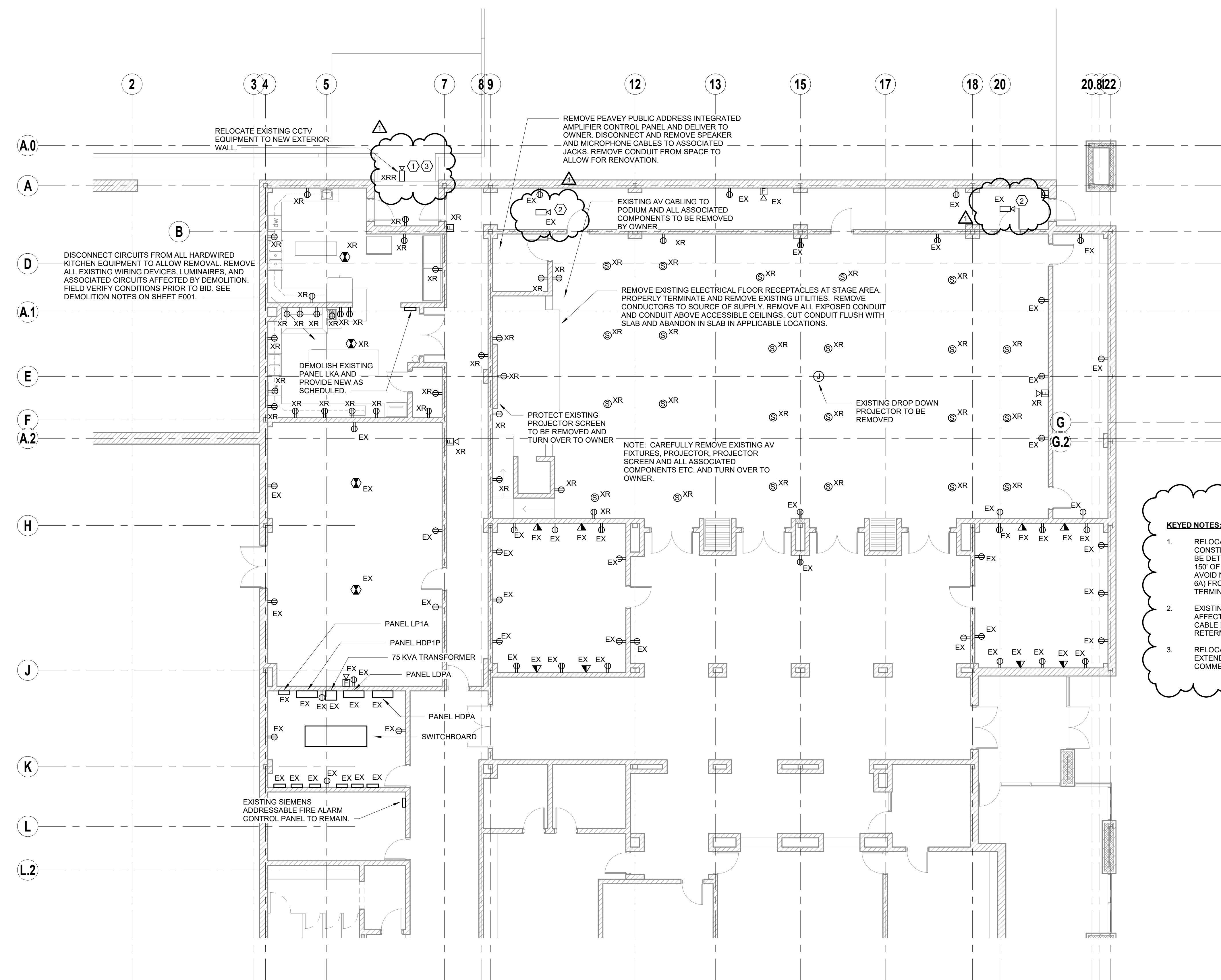
1 Floor Plan - Power & Auxiliary (Demo) 1/8" = 1'-0"
