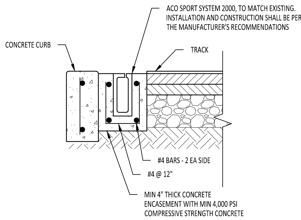
1 C203 TRENCH DRAIN DETAIL SCALE: NOT TO SCALE
