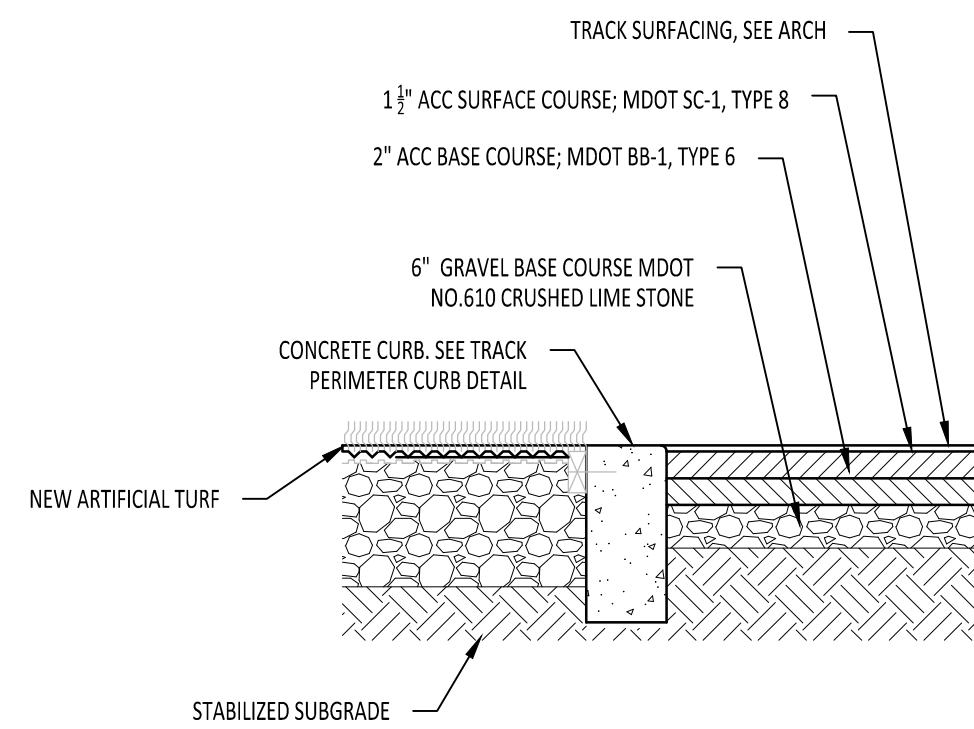
TRACK PAVING
