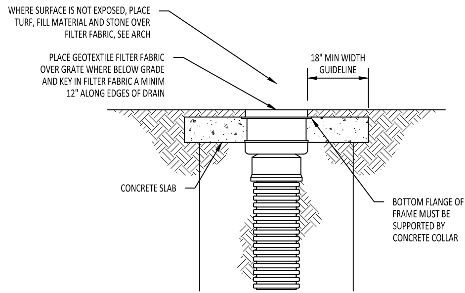
INLINE DRAIN
