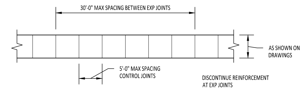
TYPICAL PLAN
