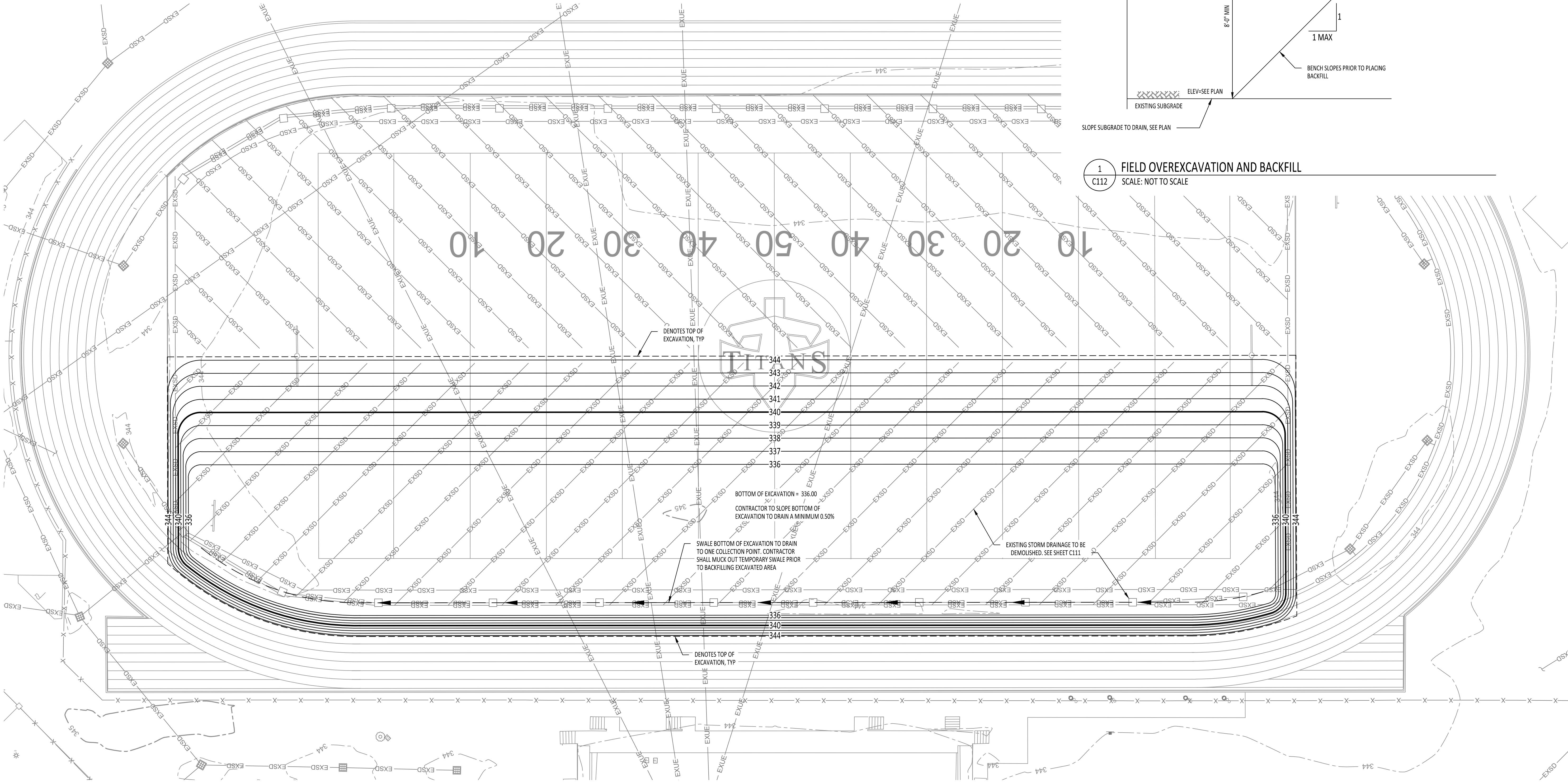
OVEREXCAVATION PLAN SCALE: 1"=20'-0"
