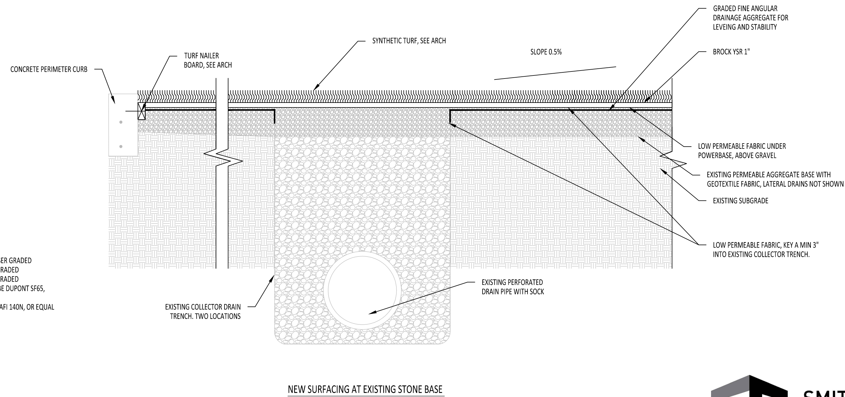
4 FIELD SECTIONS AND COLLECTOR PIPE DETAILS SCALE: NOT TO SCALE
