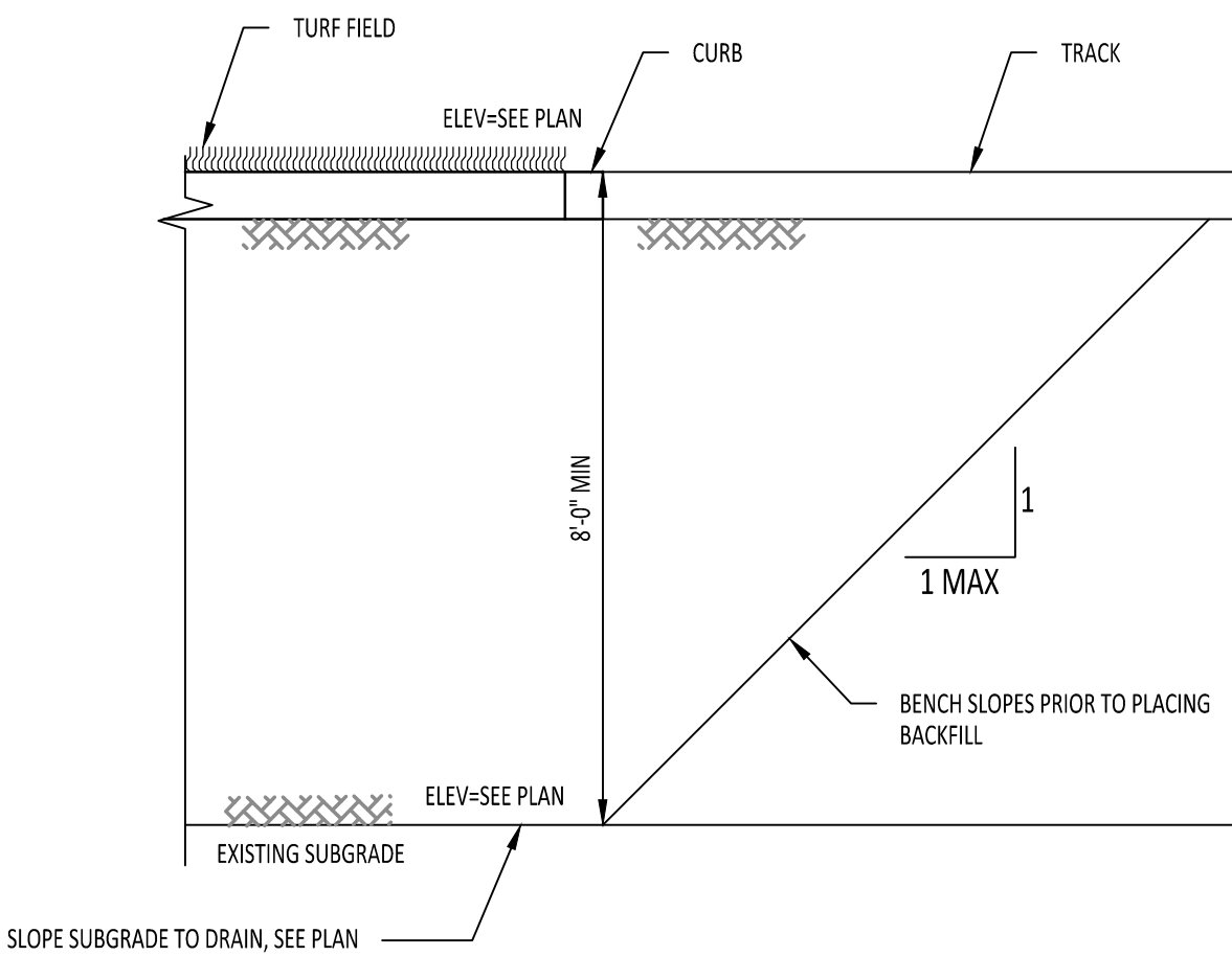
1 FIELD OVEREXCAVATION AND BACKFILL SCALE: NOT TO SCALE
