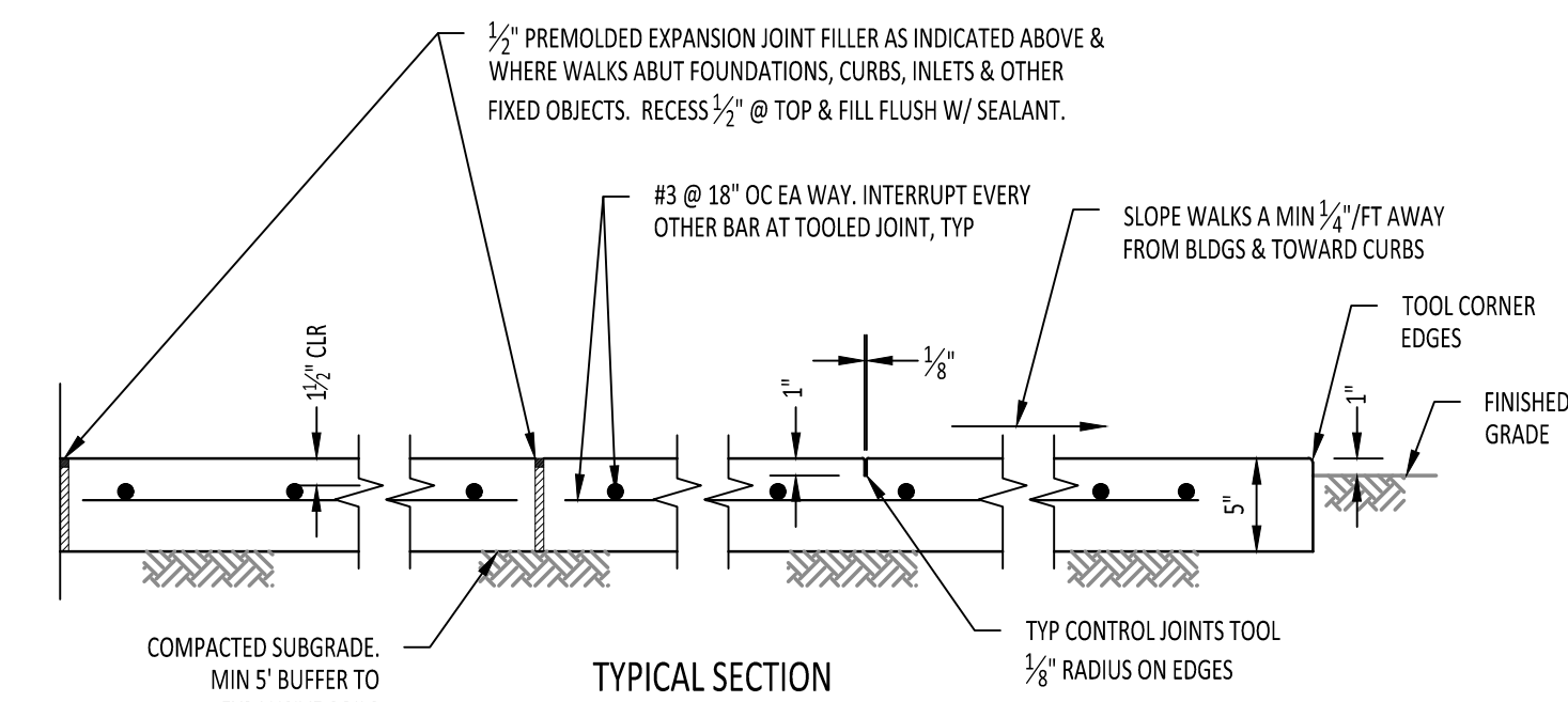
TYPICAL SECTION
