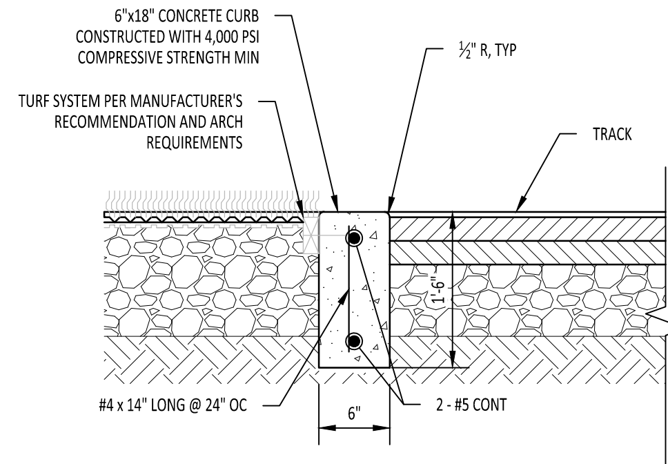
2 TRACK PERIMETER CURB SCALE: NOT TO SCALE
