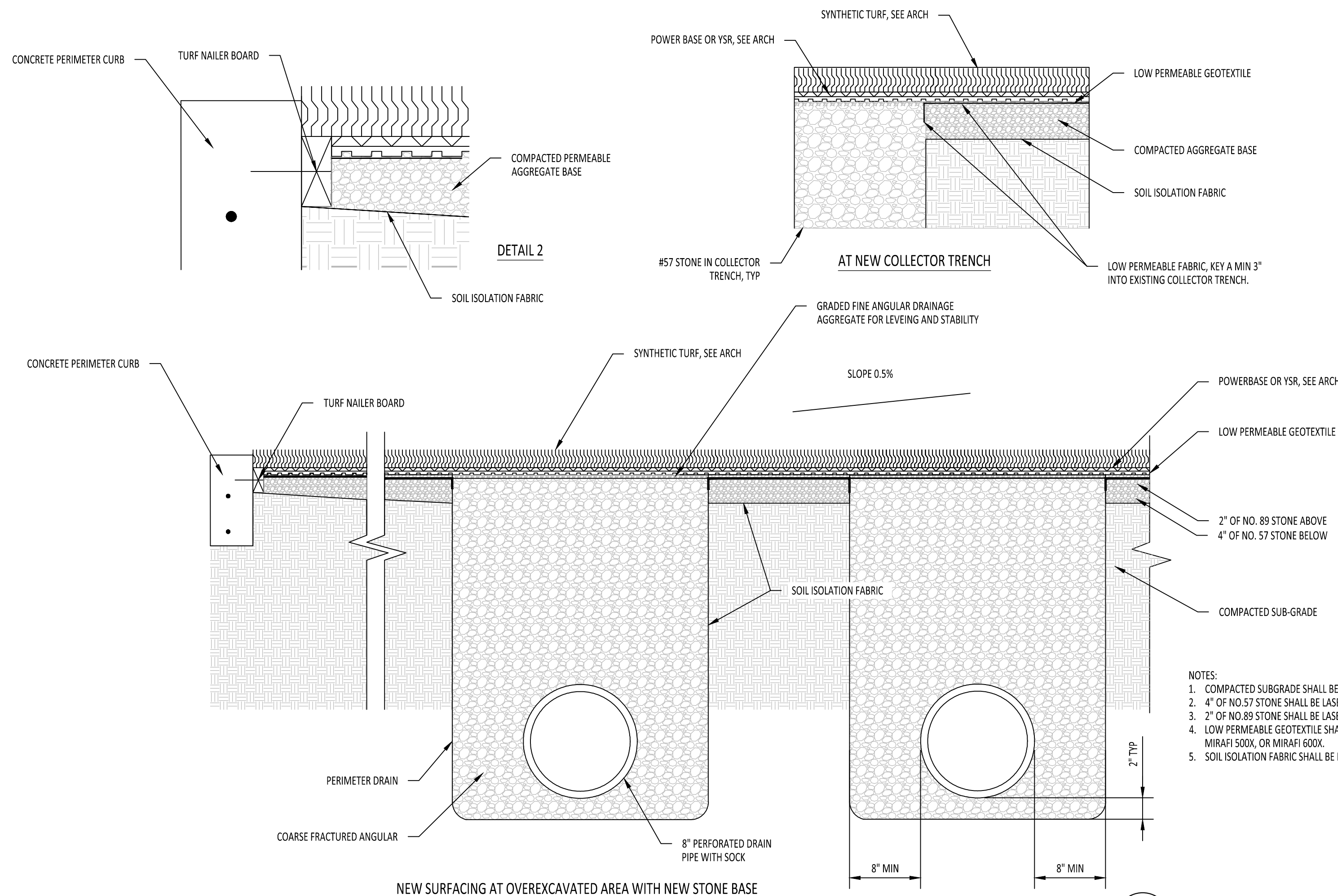
4 FIELD SECTIONS AND COLLECTOR PIPE DETAILS SCALE: NOT TO SCALE
