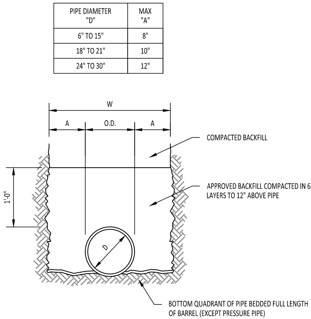
2 C203 UTILITY CONDUIT SCALE: NOT TO SCALE
